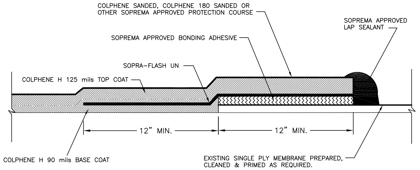
SINGLE PLY MEMBRANE OVERBURDEN NOT SHOWN
